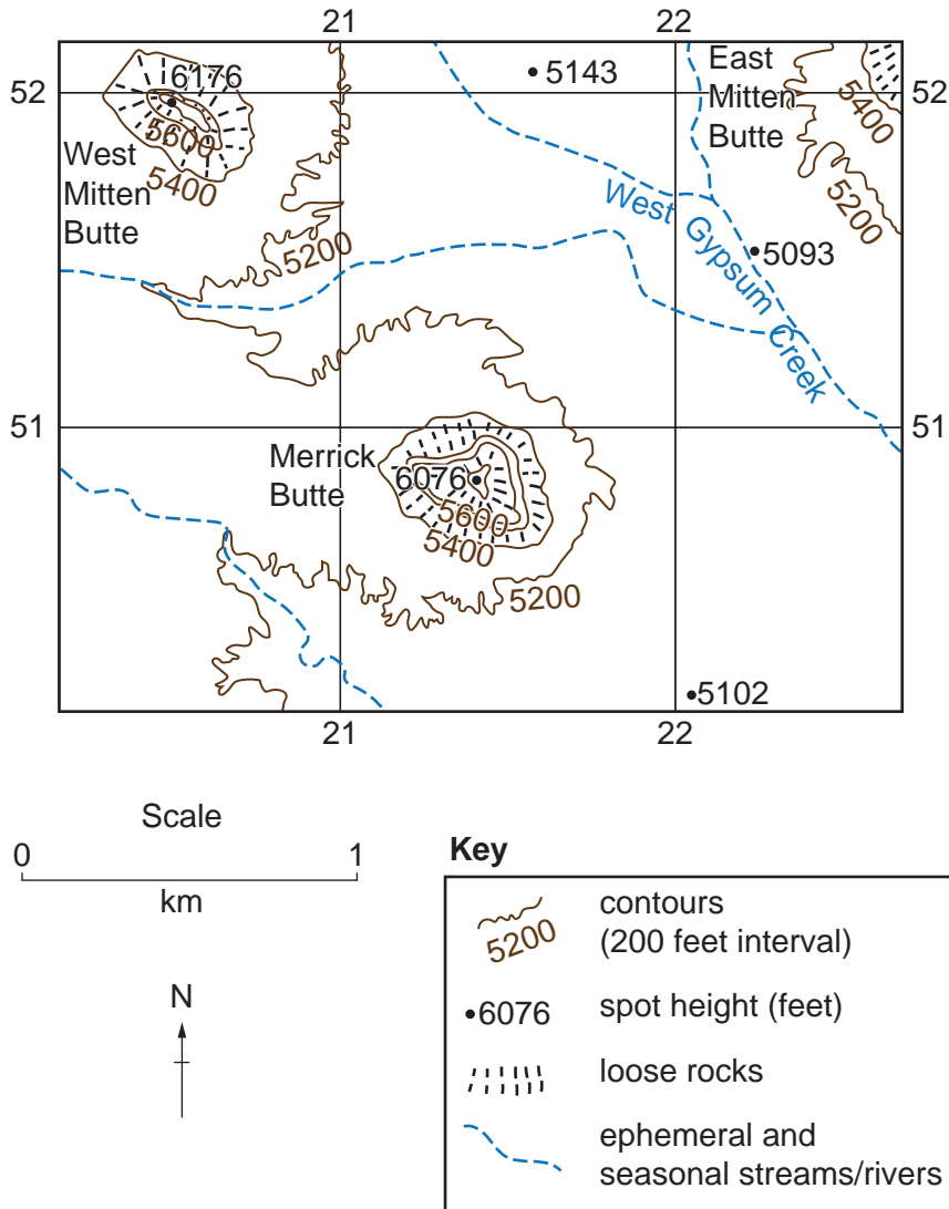
Fig. 3 – Contour map of a dryland landscape in Arizona, USA
