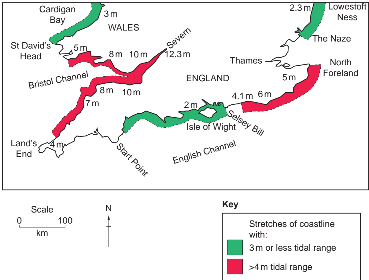
Fig. 1 – Average tidal range at the coast of southern England and Wales
