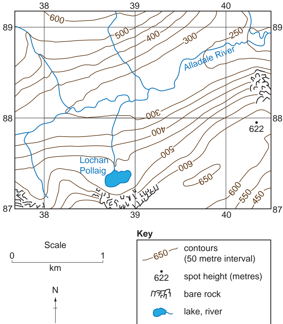
Fig. 2 – Contour map of a glaciated landscape in the North West Highlands, Scotland
